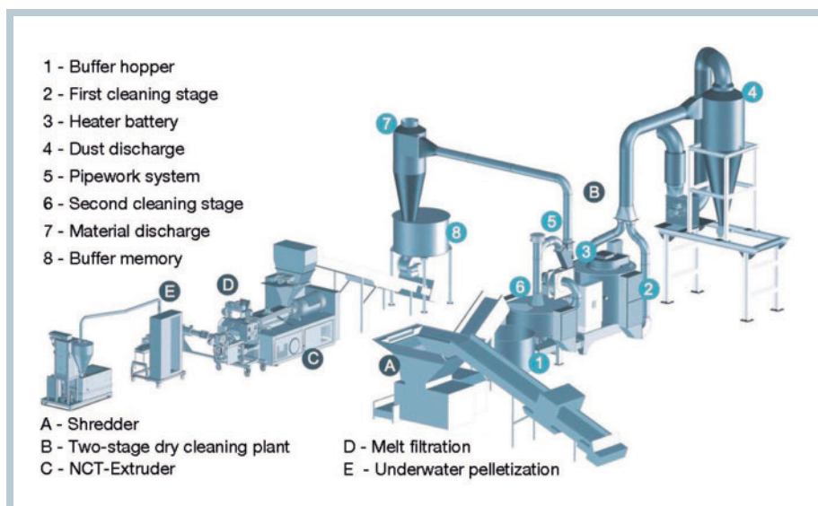
Fig. 1. Layout of the compact plant
