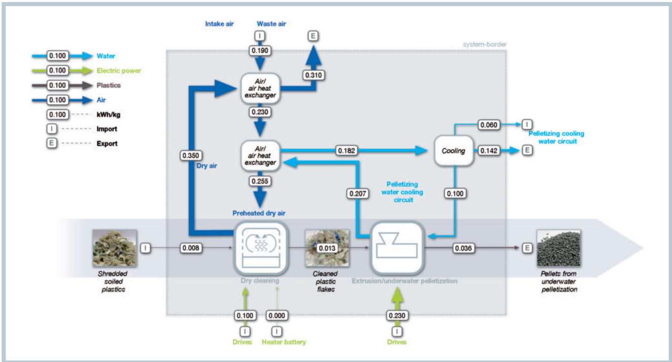
Fig. 2. Energy balance of the compact plant (fluxes in kWh/kg)
